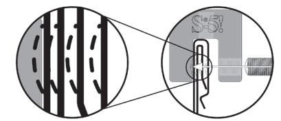
(Top) S-5-U clamp on both vertical and horizontal seams.
